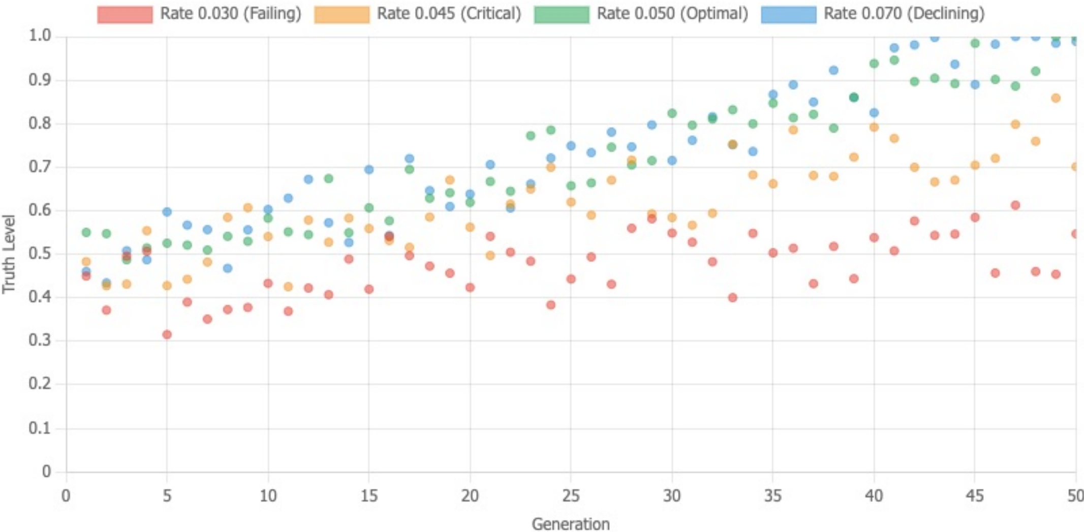
Scatter Plot: Generation vs Truth Level - Path Dependency Analysis
